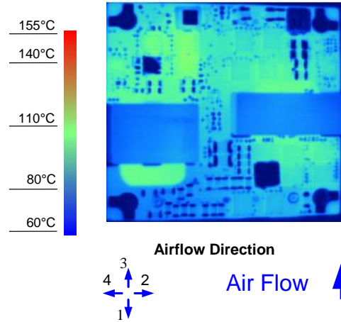
Figure 8. Thermal Image for Airflow Direction 3 (12A output, 55°C ambient, 200 LFM, typical Vin, open frame, unit soldered onto a fixture board)
