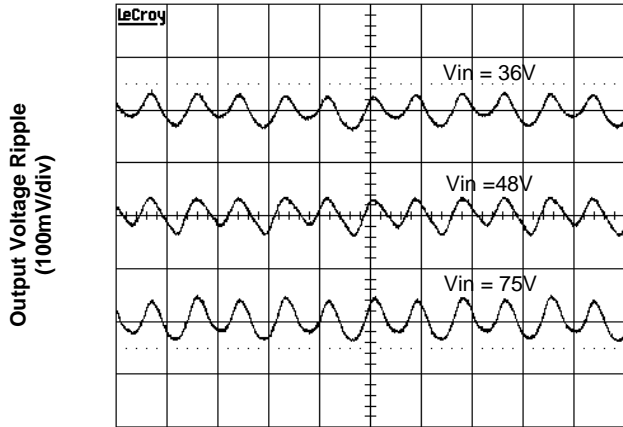
Time - t (5µs/div)
