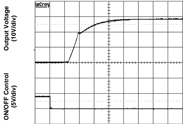
Time - t (5ms/div)
