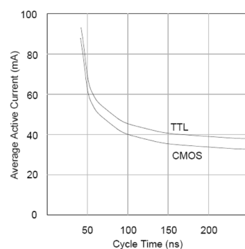
Figure 5. Current Versus Cycle Time (WRITE)
