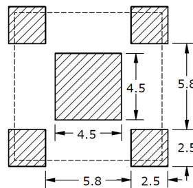
Figure 20 Recommended Soldering Footprint
